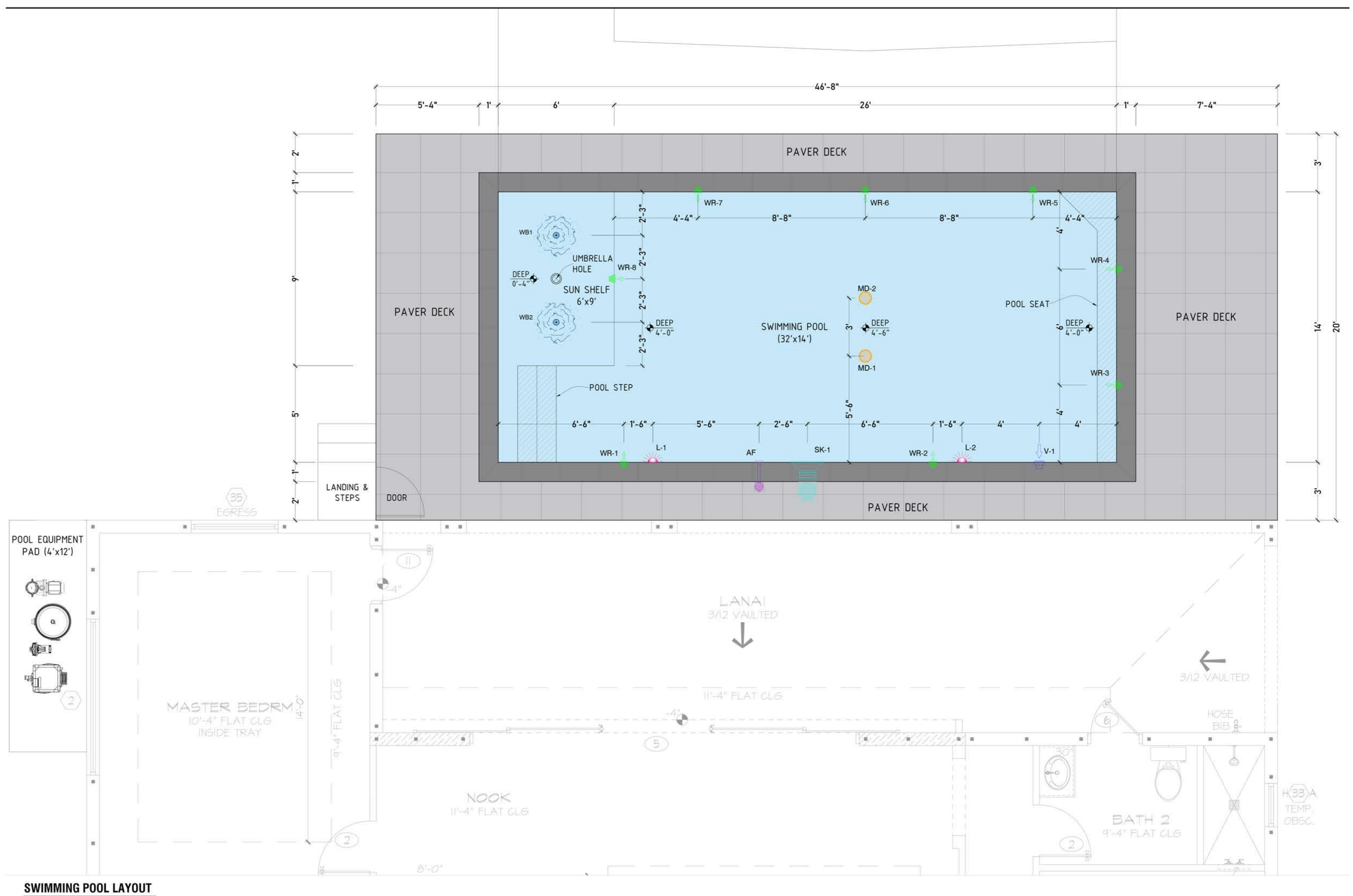
SWIMMING POOL LAYOUT
